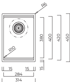
INTEGRATO Q Bar/Prep Sink
