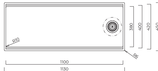
INTEGRATO Q Super Single Sink (Reversible)
