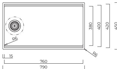
INTEGRATO Q Large Single Sink (Reversible)
