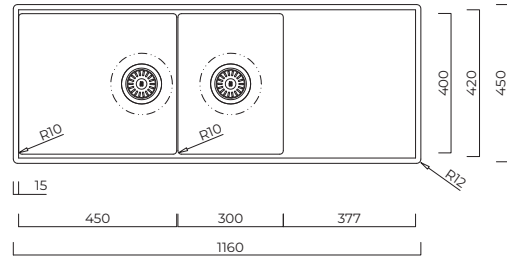
STRATUS Q Double Bowl 60 / 40 + Drainer (Reversible) SQC450DU
